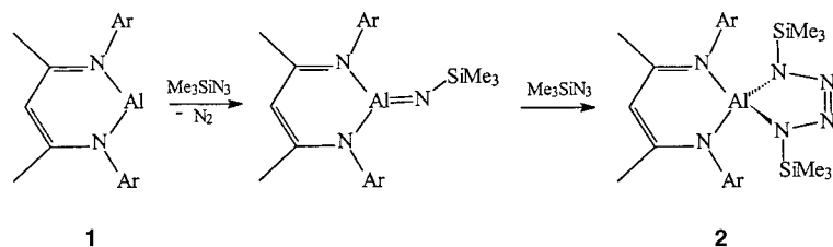
Scheme 1. Synthesis of 2 . Ar = 2,6\text{-}iPr_2C_6H_3 .
